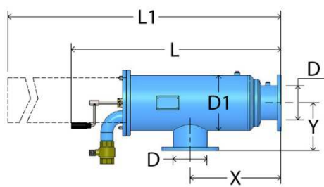
SA504B – SA508B
