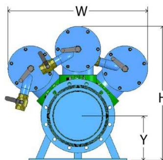
SA514B [3xSA508B]
